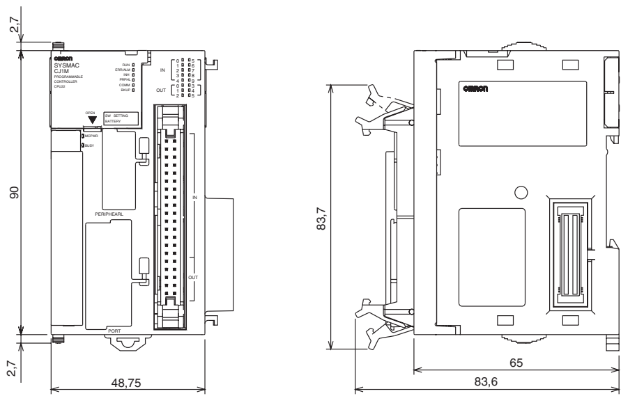
CJ1M-CPU2
