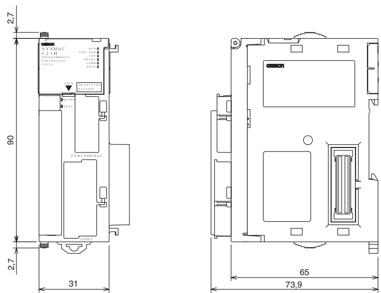
CJ1M-CPU2
